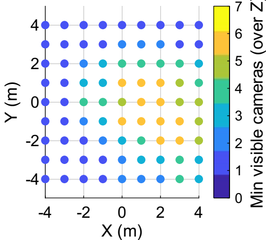
GA-best: XY worst-case
